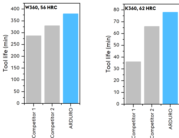
Fig. 1: Performance comparison of the new ARDURO® used with end mills, diameter 10 mm. f_z = 0.025 mm, a_p = 5 mm, a_e = 0.5 mm, max. wear mark width V_{B,max} = 0.10 mm. Cutting speed: left v_c = 95 m/min, right v_c = 65 m/min
