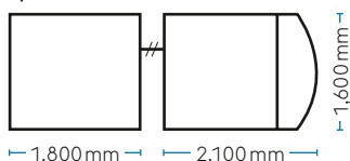
Split frame
